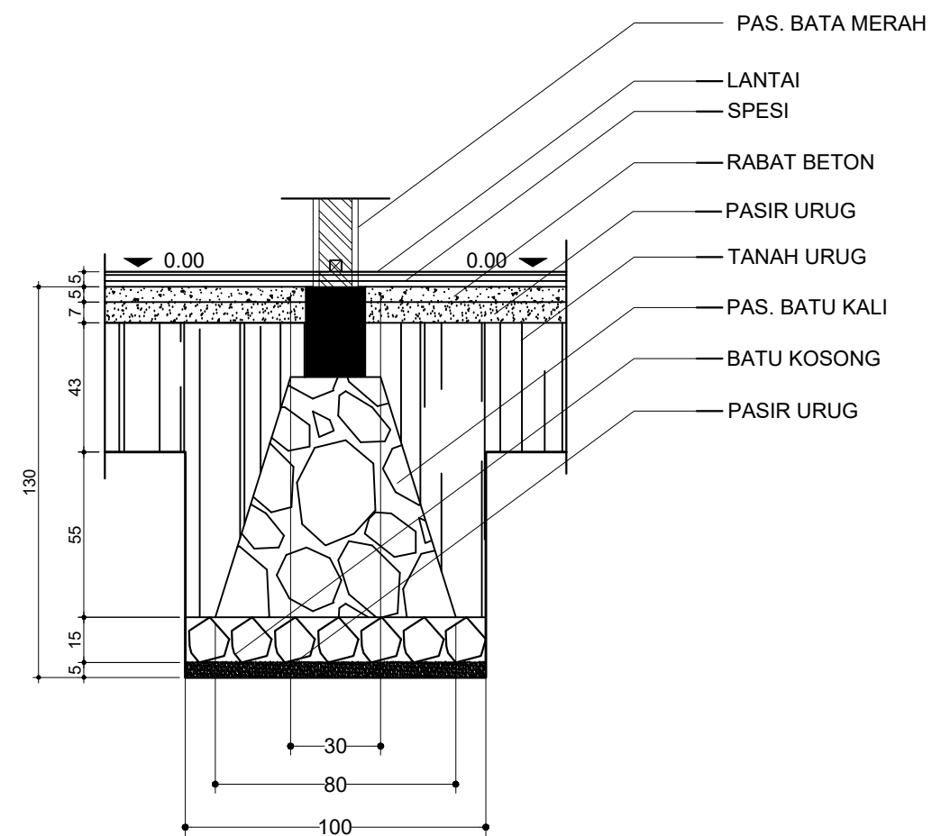
DETAIL PONDASI A SKALA 1 :20
