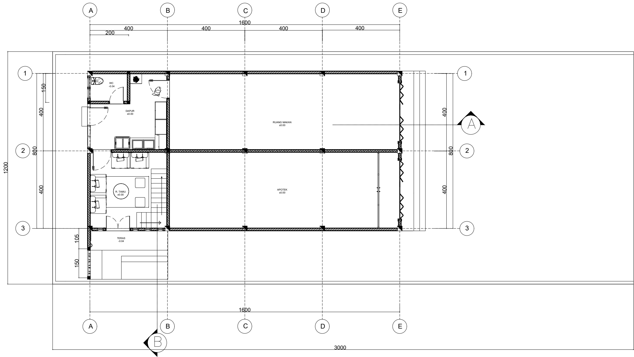
DENAH LT 1 SKALA 1:100
