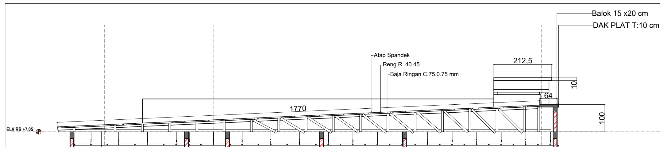
DETAIL POTONGAN ATAP A - A SKALA 1:75
